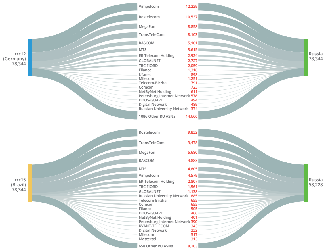
Figure 9: First Russian ASNs observed from Germany (top) and Brazil (bottom), with the number of prefixes passing through each ASN labelled.
